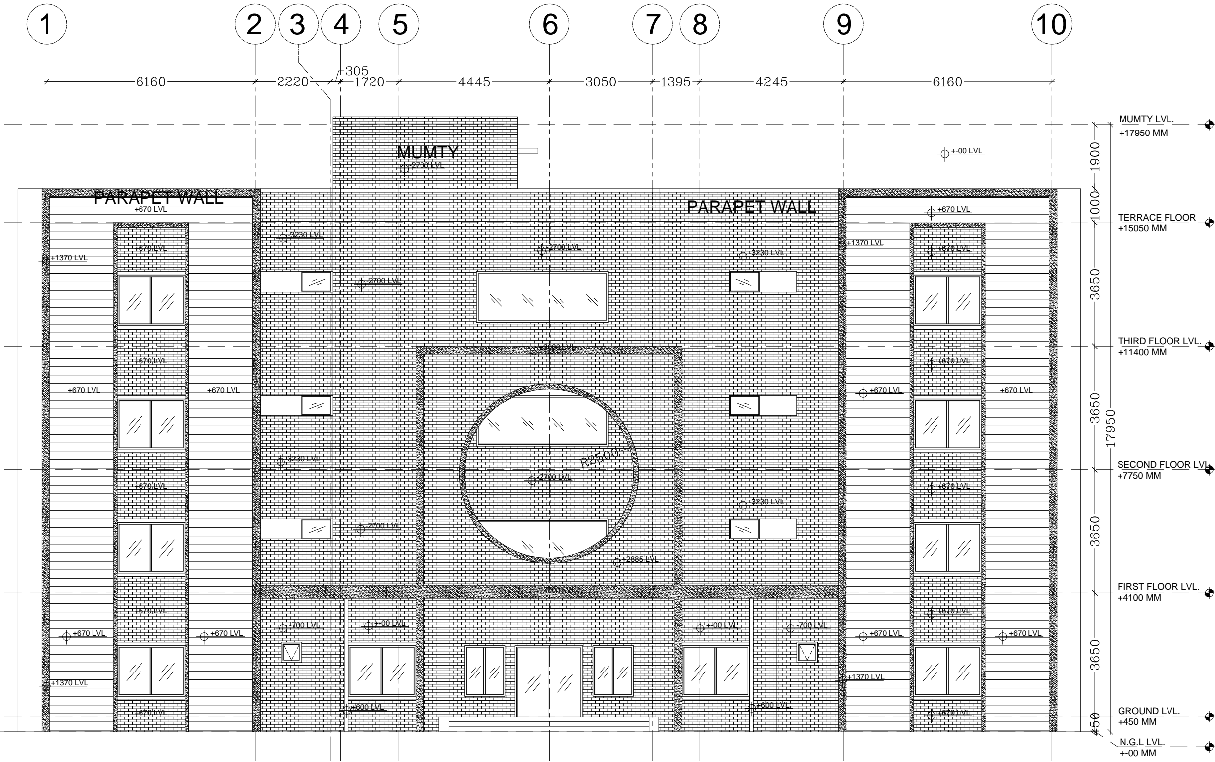
FRONT ELEVATION
